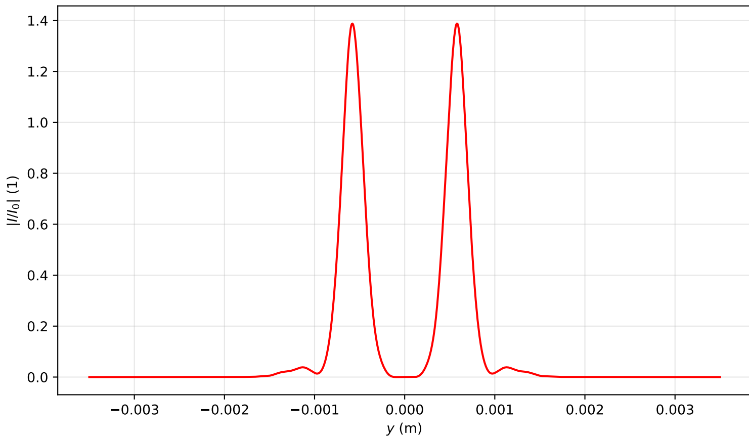
Intensity profile I(x=0, y, z=0.876)/I_0 , P_{in}=7.0P_{cr} , artificial time
